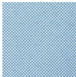
A 44 pacific
