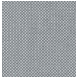
A 41 cloud
